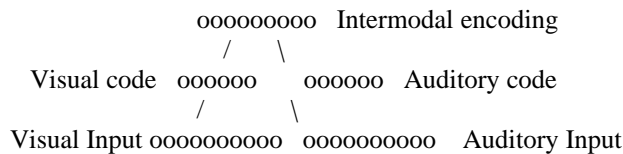
Figure 3. Automatically learned inter-modal encoding. The inputs and outputs of the network in Figure 2 have been overlain in this diagram, and correspond to the lower left and lower right parts. The final layer is a joint encoding of the hidden unit layers of the modality-specific codes.
